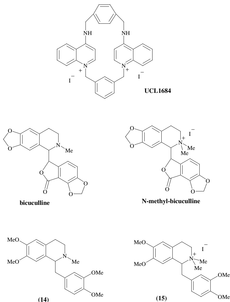
Figure 1. Chemical structures of UCL 1684, bicuculline, N -methyl-bicuculline, laudanosine 14 and N -methyl-laudanosine iodide 15 .
