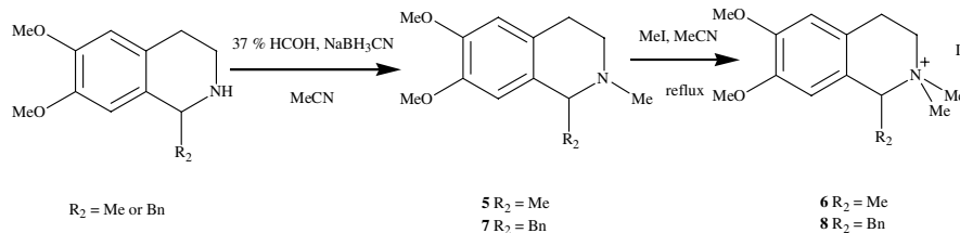
Scheme 2. Preparation of 1-substituted-2,2-dimethyl-1,2,3,4-tetrahydroisoquinolinium derivatives.
