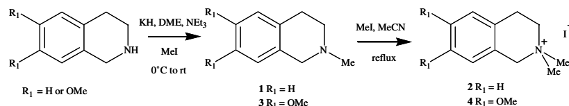
Scheme 1. Preparation of 2,2-dimethyl-1,2,3,4-tetrahydroisoquinolinium analogues.
