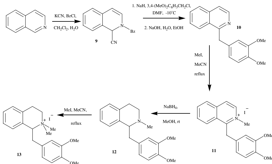
Scheme 3. Synthesis of 1-(3,4-dimethoxybenzyl)-2,2-dimethyl-1,2,3,4-tetrahydroisoquinolinium iodide 13 .
