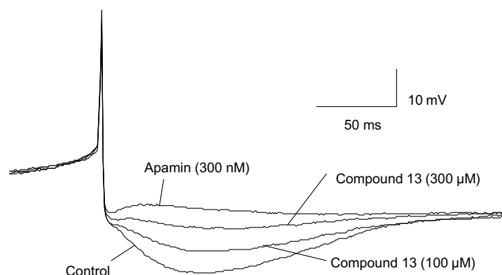
Figure 2. Effect of increasing concentrations of compound 13 on the AHP of midbrain dopaminergic neurons. While 100% blockade of the AHP is obtained with 300 nM apamin, 67.3% blockade is obtained with 300 μM compound 13 . Each trace is the mean of four sweeps. Action potentials are truncated.
